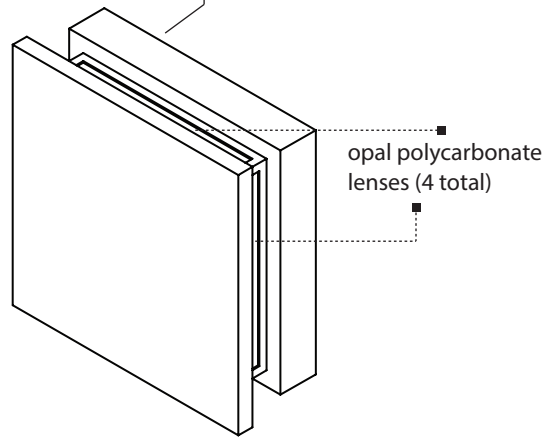
Iso view
