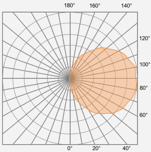
Front Light
