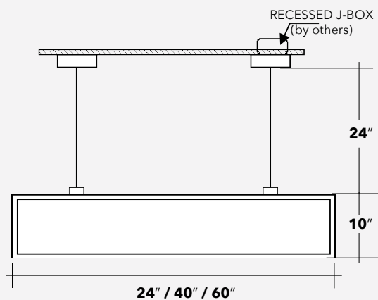
2AC24 Mounting
