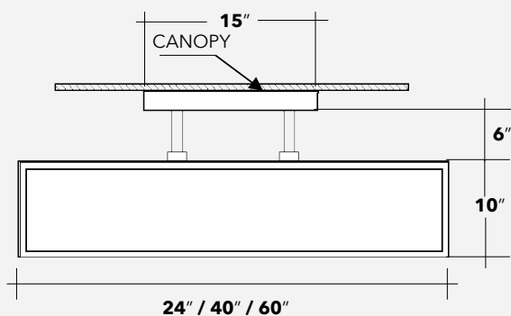
2P6 Mounting
